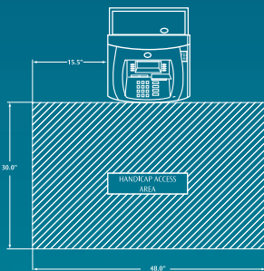
ATM INSTALLATION SPACE REQUIREMENTS FOR ADA COMPLIANCE
